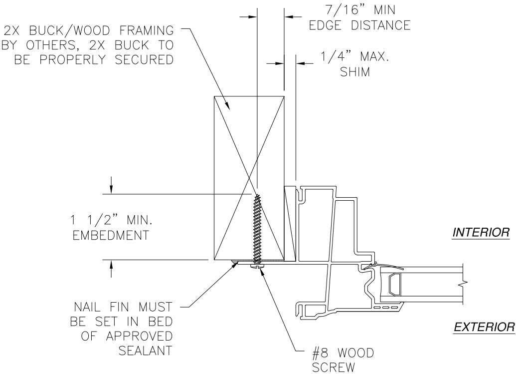
JAMB INSTALLATION 2X BUCK/WOOD FRAMING
